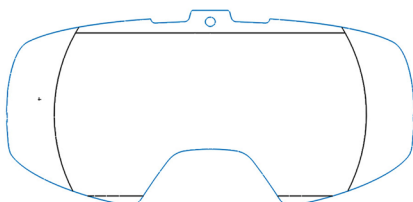
FIGURE 1: NIJ STANDARD-0104.02 VISUAL AREA IN BLACK RELATIVE TO REVISION VISOR IN BLUE
